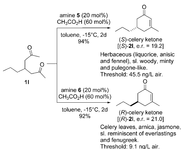
Scheme 1. Synthesis of both enantiomers of celery ketone ( 2 ).
